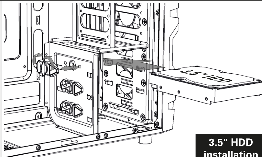
3.5" device installation
